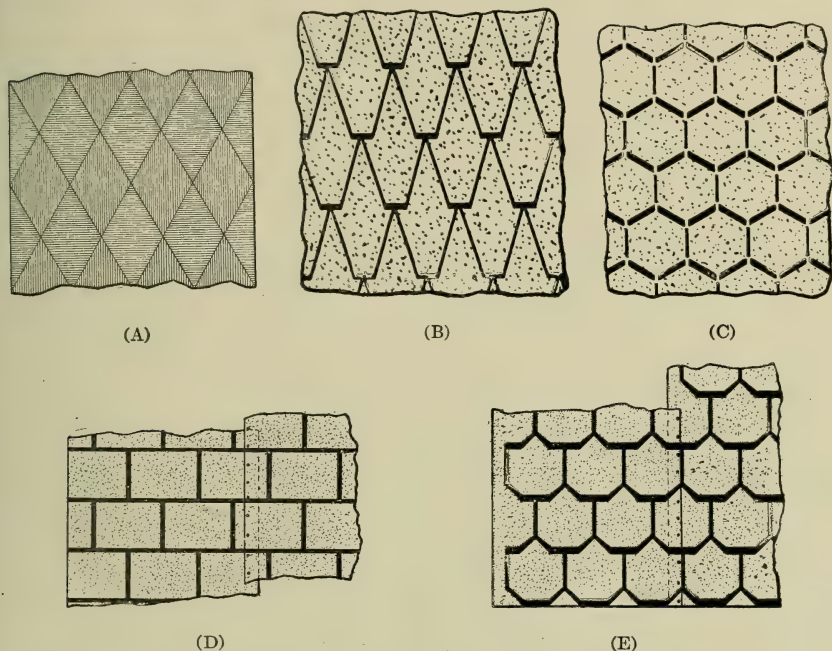
FIG. 134.—Roll Roofings Finished in an Ornamental Surface.
